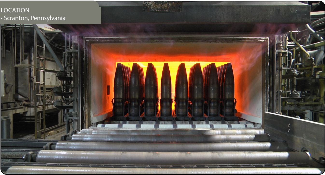
Projectiles cartridge case are heated in the heat treat shop as a part of the production process at Scranton Army Ammunition Plant. (U.S. Army photo by Dori Whipple)
